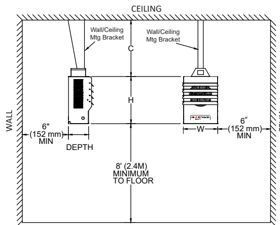
FIG. 2 HORIZONTAL CEILING MOUNT WITH MTG ARM
