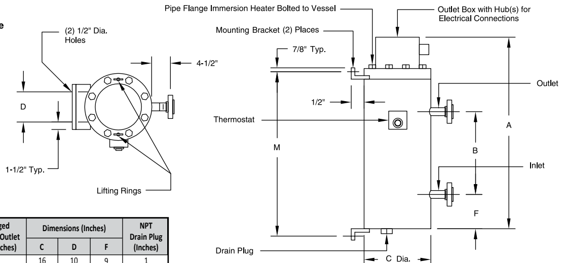
Figure 3 10", 12" & 16" Flange Construction
