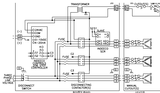
Open Coil
