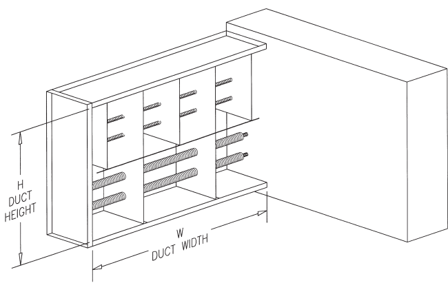
Figure 70. Flanged Duct Heater
