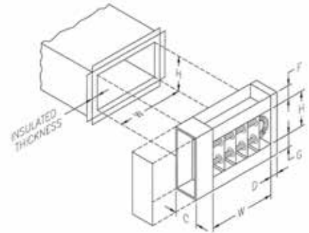
Figure 65. Installation of flange type heater in lined duct
