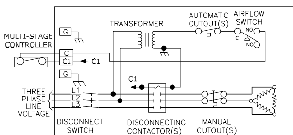
Open Coil
