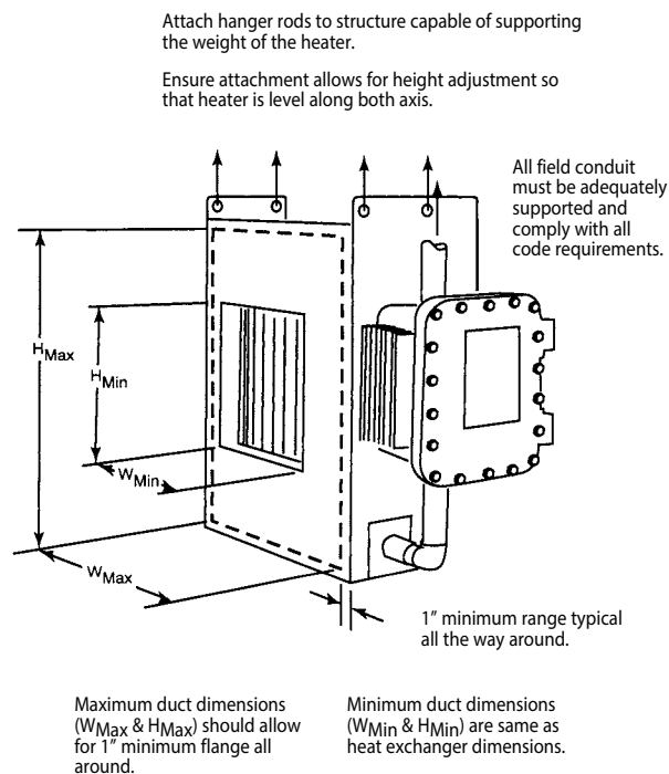
Figure 78. ULTRA-SAFE™ Mounting Configuration
