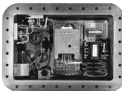
Figure 88. Control Enclosure
