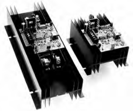
Figure 34. A & B Series for indoor use
