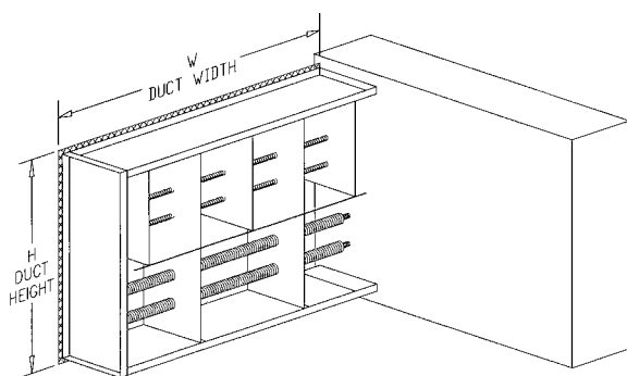
Figure 69. Slip-in Duct Heater
