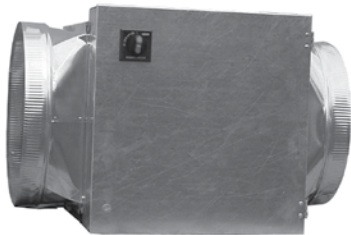
Figure 52. Open Coil heater with round duct transitions.
