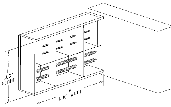
Figure 70. Flanged Duct Heater
