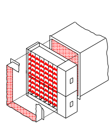
Fig. 3 - Installation drawing of two stacked sections in a duct.
